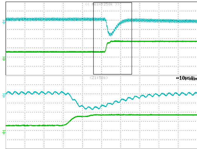
Figure 15: Transient Response
