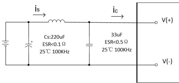
Figure 17: Test Setup Diagram for Input Ripple Current
