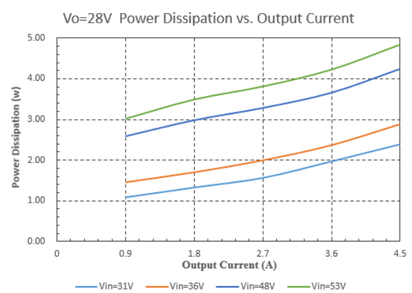
Figure 8: Power Dissipation vs. Output Current(Vo=28V)
