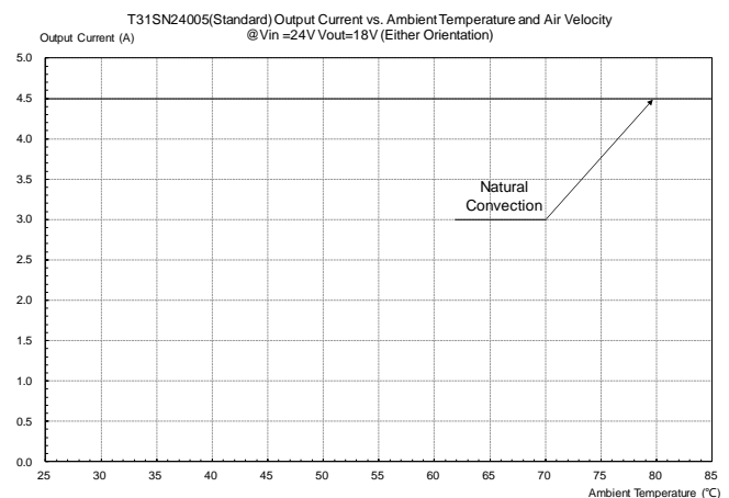
Figure 26: Output current vs. ambient temperature and air velocity @ V_{in}=24V , V_{out}=18V (Either Orientation, Open Frame)
