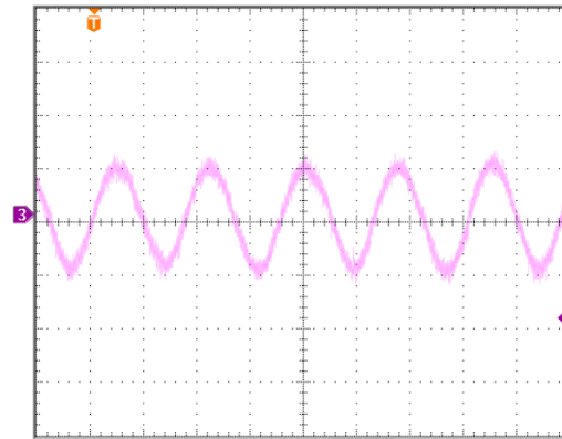
Figure 19: Input Reflected Ripple Current, i_s , through a 12\mu H source inductor at 48Vdc input voltage, 15Vdc output voltage and max load current (100mA/div, 2us/div).
