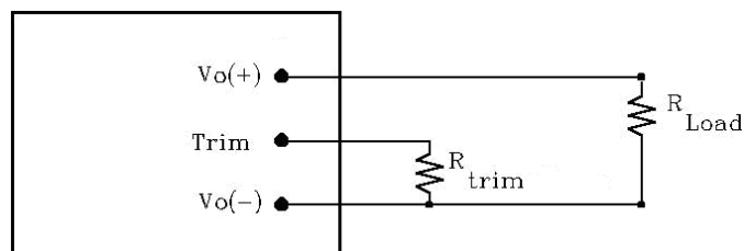
Figure 23: Circuit Configuration for Trim (decrease output voltage)
