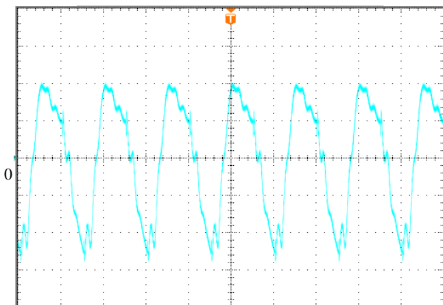
Output voltage ripple at nominal input voltage and max load current (20mV/div, 2μs/div) Load cap: 10μF, tantalum capacitor and 1μF ceramic capacitor. Bandwidth: 20MHz.
