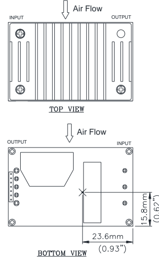
Figure 20: Hot spot 2 temperature measurement location
