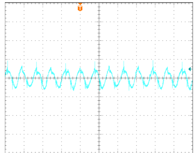
Figure 12: Output Voltage Ripple and Noise at nominal input voltage and max load current (25 mV/div, 4us/div) Load cap: 820uF Oscon, 33uF*6 MLCC, 1μF Ceramic, 10μF Tantalum. Bandwidth: 20MHz.
