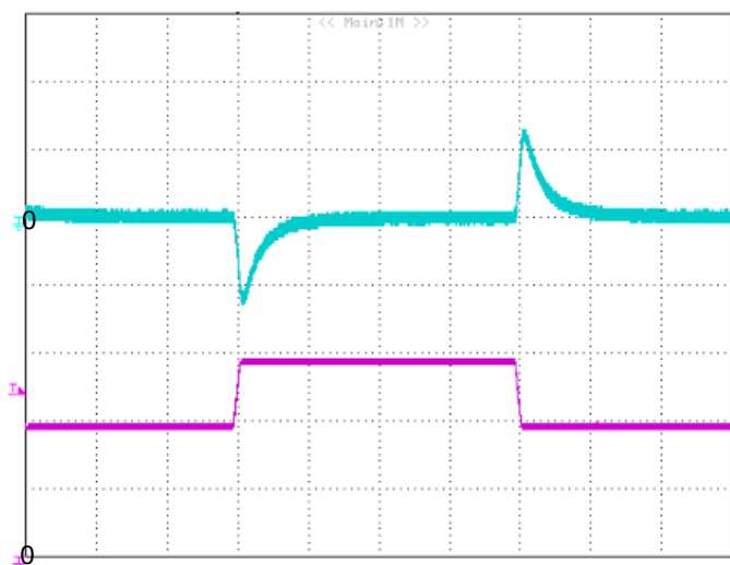
Figure 6: Output voltage response to step-change in load current (50%-75%-50% of I_o max; di/dt = 0.1A/\mu s ; V_{in} is 24V). Load cap: 10 \mu F tantalum capacitor and 1 \mu F ceramic capacitor. Top Trace: V_{out} (0.5V/div, 500us/div), Bottom Trace: I_{out} (5A/div). Scope measurement should be made using a BNC cable (length shorter than 20 inches). Position the load between 51 mm to 76 mm (2 inches to 3 inches) from the module
