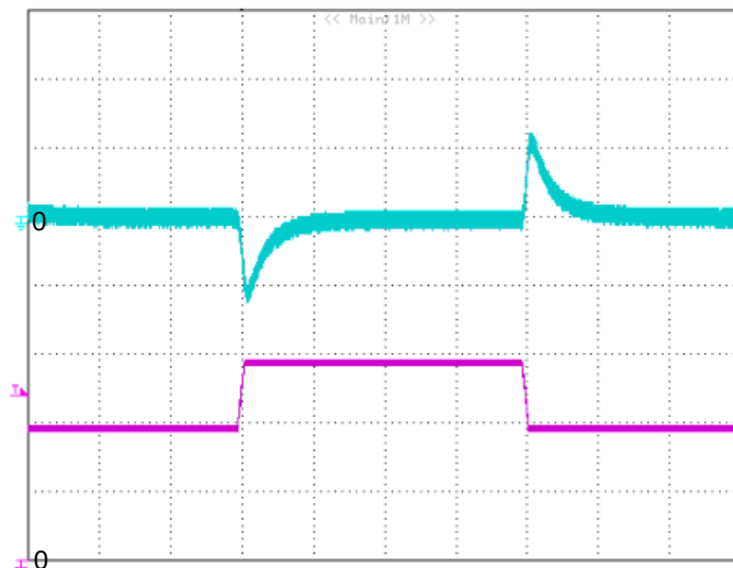
Figure 7: Output voltage response to step-change in load current (50%-75%-50% of I_o max; di/dt = 0.1A/\mu s ; V_{in} is 48V). Load cap: 10 \mu F tantalum capacitor and 1 \mu F ceramic capacitor. Top Trace: V_{out} (0.5V/div, 500us/div), Bottom Trace: I_{out} (5A/div). Scope measurement should be made using a BNC cable (length shorter than 20 inches). Position the load between 51 mm to 76 mm (2 inches to 3 inches) from the module
