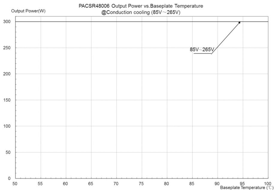
Figure 13: Thermal derating curves
