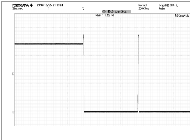
Figure 7: Output OVP at 110/220Vac, 6.3A Iout Vout: 10V/div, 500ms/div
