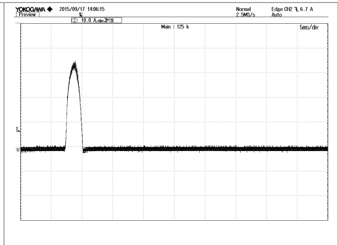
Figure 8: Inrush current @ Vin=220Vac Iin:10A/div, 5ms/div;
