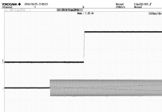
Figure 5: V_{out} start up at 220Vac, 6.3A I_{out} , TOP: V_{out} , 20V/div, 500mS/div BOTTOM: V_{in} , 500V/div, 500mS/div
