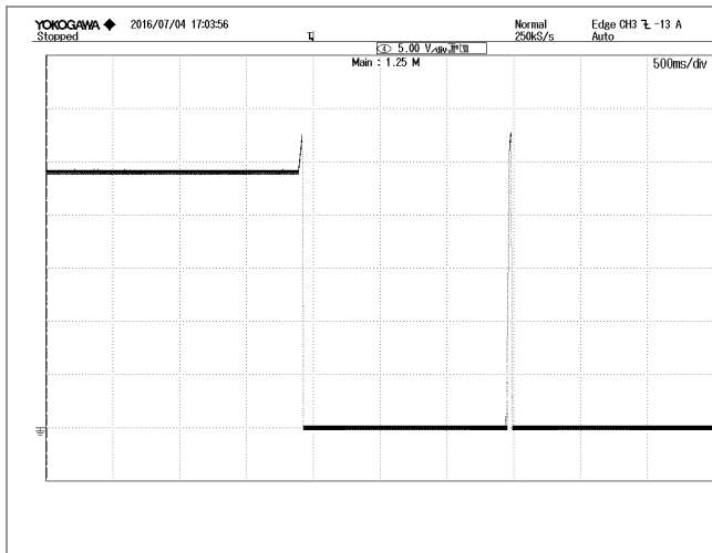
Figure 7: Output over voltage protection at 110/220Vac, 21A Iout, VOUT: 5V/div, 500mS/div
