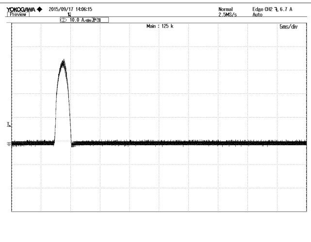
Figure 8: Inrush current @ Vin=220Vac lin: 10A/div, 5mS/div;
