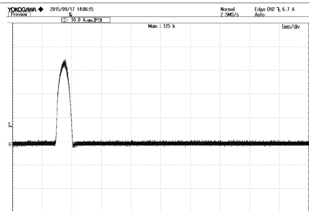
Figure 8: Inrush current @ Vin=220Vac CH2:lin, 10A/div, 5mS/div;
