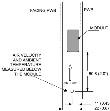
Figure 32: Wind tunnel test setup
