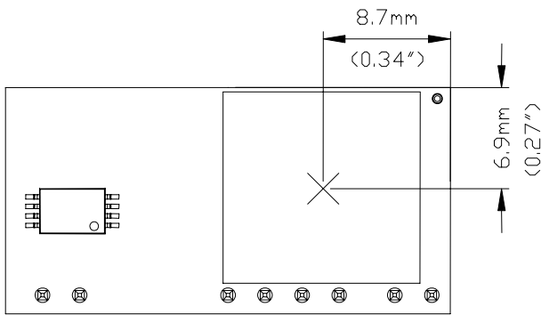
Figure 39: Temperature measurement location * The allowed maximum hot spot temperature is defined at 125°C
