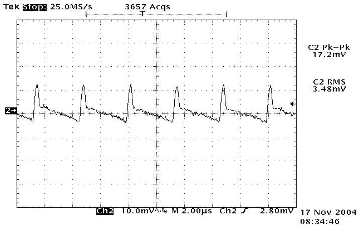
Figure 7: Output ripple & noise at 12Vin, 0.9V/6A out
