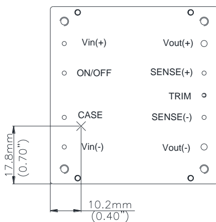
Figure 18: *Hot spot on Base Plate temperature measurement location viewed from top side. The allowed maximum hot spot temperature is 95°C at 48Vin @550W.
