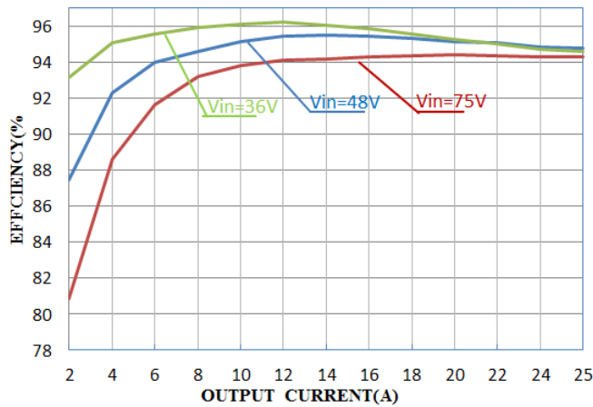
Figure 1: Efficiency vs. load current for 36V, 48V, and 75V input voltage at 25^{\circ}\text{C} .
