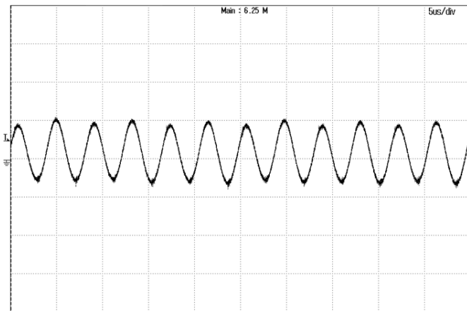
Figure 12: Input reflected ripple current, i_s , through a 12\mu\text{H} source inductor at nominal input voltage and max load current ( 100\text{mA/div} \cdot 5\text{us/div} ).
