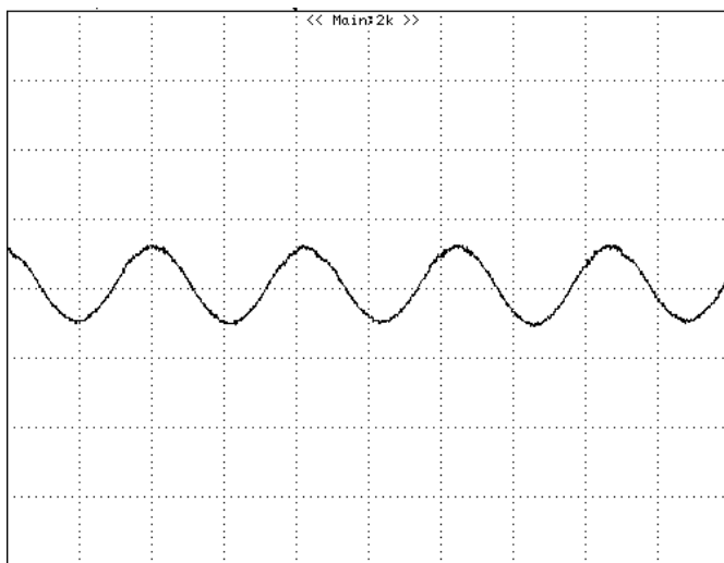
Figure 14: Output voltage ripple at nominal input voltage and max load current ( 100\text{mV/div}, 2\text{us/div} ) Load capacitance: 50\mu\text{F} ceramic capacitor and low ESR 1350\mu\text{F} Electrolytic Capacitor. Bandwidth: 20\text{MHz} .
