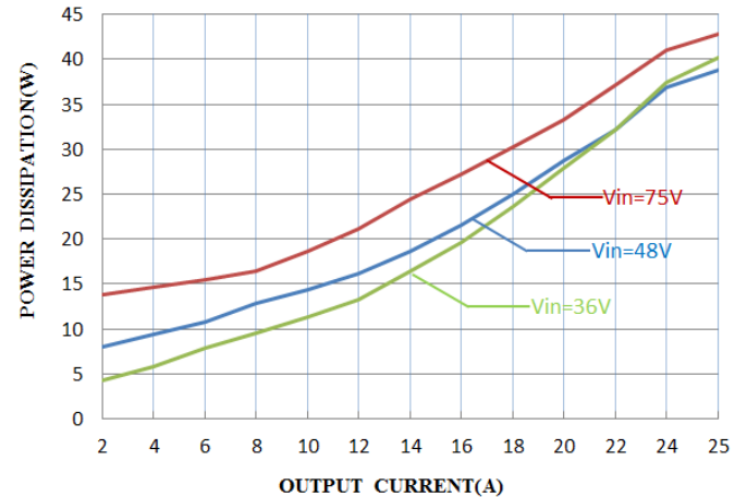
Figure 2: Power dissipation vs. load current for 36V, 48V, and 75V input voltage at 25^{\circ}\text{C} .
