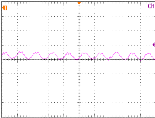
Figure 12: Input reflected ripple current, i_s , through a 12\mu\text{H} source inductor at nominal input voltage and max load current (25mA/div, 4us/div).
