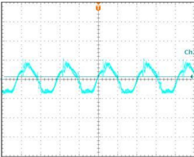
Figure 14: Output voltage ripple at nominal input voltage and max load current (50 mV/div, 2us/div) Load capacitance: 50\mu\text{F} ceramic capacitor and 1000\mu\text{F} Electrolytic Capacitor. Bandwidth: 20 MHz.
