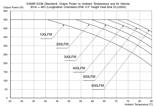
Figure 22: Output Power vs. Ambient Temperature and Air Velocity @ Vin = 48V (Longitudinal Orientation, Airflow from Input to Output, With 0.5 inch Height Heat Sink ELL050A)
