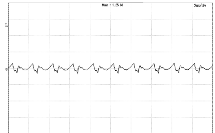
Figure 9: Input Terminal Ripple Current, i_c , at max output current and nominal input voltage with 12µH source impedance and 100µF electrolytic capacitor (500 mA/div, 2us/div).
