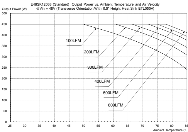
Figure 20: Output Power vs. Ambient Temperature and Air Velocity @ Vin = 48V (Transverse Orientation, Airflow from Vin+ to Vin-, With 0.5 inch Height Heat Sink ETL050A)
