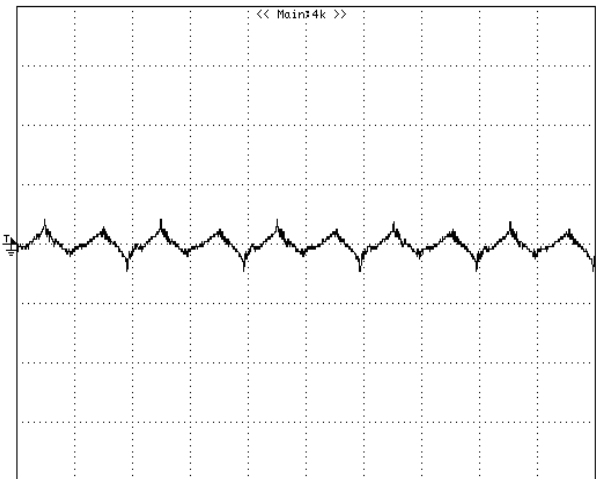
Figure 14: Output voltage ripple at nominal input voltage and rated load current ( I_o=30A )(50 mV/div, 2 \mu s/div) Load capacitance: 1 \mu F ceramic capacitor and 10 \mu F tantalum capacitor. Bandwidth: 20 MHz. Scope measurements should be made using a BNC cable (length shorter than 20 inches). Position the load between 51 mm to 76 mm (2 inches to 3 inches) from the module.
