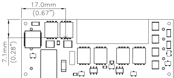
Figure 21: Case temperature measurement location.
