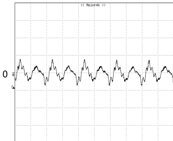
Figure 14: Output voltage ripple at nominal input voltage and rated load current ( I_o=35\text{A} ) ( 20\text{ mV/div} , 2\mu\text{s/div} ). Load capacitance: 1\mu\text{F} ceramic capacitor and 10\mu\text{F} tantalum capacitor. Bandwidth: 20\text{ MHz} . Scope measurements should be made using a BNC cable (length shorter than 20 inches). Position the load between 51 mm to 76 mm (2 inches to 3 inches) from the module.
