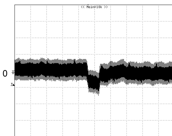
Figure 9: Output voltage response to step-change in load current (50%-75% of I_o , max; di/dt = 0.1A/\mu s ). Load cap: 10\mu F , tantalum capacitor and 1\mu F ceramic capacitor. Trace: V_{out} (20mV/div, 100us/div), Scope measurement should be made using a BNC cable (length shorter than 20 inches). Position the load between 51 mm to 76 mm (2 inches to 3 inches) from the module..
