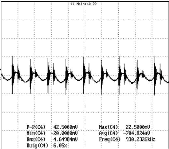
Figure 15: Output voltage ripple at nominal input voltage and rated load current ( I_o=10A )(20 mV/div, 2us/div) Load capacitance: 1 \mu F ceramic capacitor and 10 \mu F tantalum capacitor. Bandwidth: 20 MHz. Scope measurements should be made using a BNC cable (length shorter than 20 inches). Position the load between 51 mm to 76 mm (2 inches to 3 inches) from the module.
