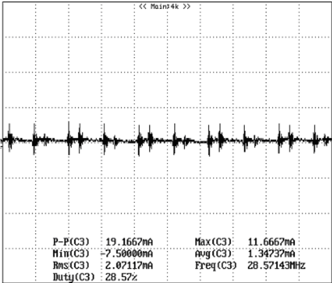
Figure 13: Input reflected ripple current, i_s , through a 12 \mu H source inductor at nominal input voltage and rated load current (20 mA/div, 2us/div).
