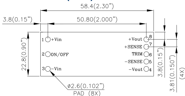
RECOMENDED P.W.B. PAD LAYOUT
