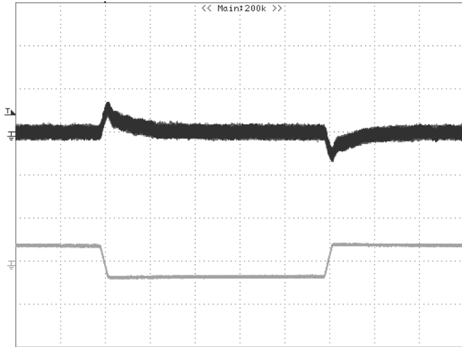
Figure 8: Output voltage response to step-change in load current (75%-50%-75% of I_{o, \text{max}} ; di/dt = 0.1\text{A}/\mu\text{s} ). Load cap: 10\mu\text{F} , tantalum capacitor and 1\mu\text{F} ceramic capacitor. Top Trace: V_{\text{out}} (100mV/div, 200us/div), Bottom Trace: I_{\text{out}} (5A/div). Scope measurement should be made using a BNC cable (length shorter than 20 inches). Position the load between 51 mm to 76 mm (2 inches to 3 inches) from the module
