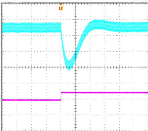
Figure 6: Transient Response (V_{in}=48V, 1A/\mu s\ step\ change\ in\ load\ from\ 50\% \ to\ 75\% \ of\ I_{o,\ max}) V_{out} (top trace): 200mV/div, 400us/div; I_{out} (bottom trace): 5A/div. Scope measurement should be made using a BNC cable (length shorter than 20 inches). Position the load between 51 mm to 76 mm (2 inches to 3 inches) from the module 470uF Oscon Cap and 11uF Ceramic Cap
