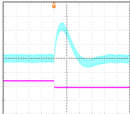
Figure 7: Transient Response (V_{in}=48V, 1A/\mu s\ step\ change\ in\ load\ from\ 75\% \ to\ 50\% \ of\ I_{o,\ max}) V_{out} (top trace):200mV/div, 400us/div; I_{out} (bottom trace): 5A/div. Scope measurement should be made using a BNC cable (length shorter than 20 inches). Position the load between 51 mm to 76 mm (2 inches to 3 inches) from the module 470uF Oscon cap and 11uF Ceramic Cap
