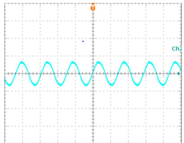
Figure 11: Output Voltage Ripple and Noise at nominal input voltage and max load current (50 mV/div, 2us/div) Load cap: 470uF Oscon cap. Bandwidth: 20MHz.
