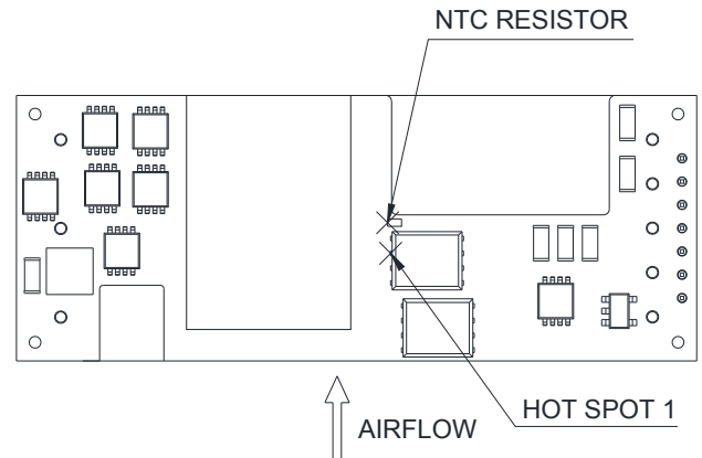
Figure 20: * Hot spot 1 & NTC resistor temperature measured points, the allowed maximum hot spot 1 temperature is defined at 116 °C.
