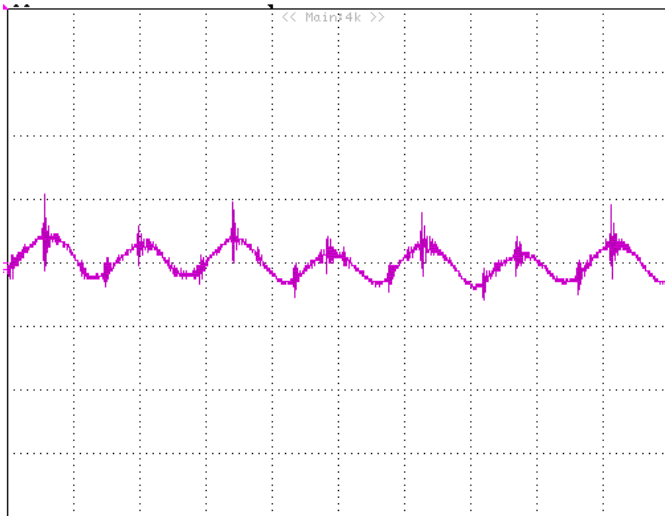
Figure 12: Input reflected ripple current, i_s , through a 12\mu\text{H} source inductor at nominal input voltage and rated load current (20mV/div, 2us/div).
