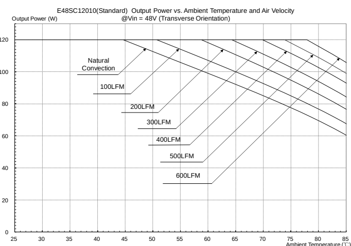
Figure 20: Output power vs. ambient temperature and air velocity @ Vin=48V(Transverse Orientation, airflow from Vin+ to Vin-, without heat spreader)
