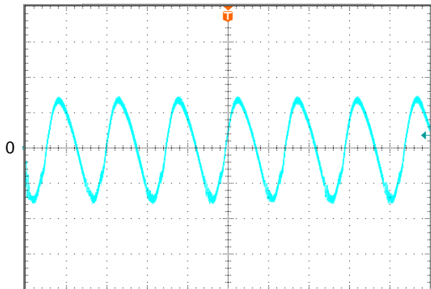
Figure 12: Output voltage ripple at nominal input voltage ( V_{in}=48V ) and rated load current ( I_o=9A ) (20mV/div, 2us/div). Load capacitance: 1 \mu F ceramic capacitor and 10 \mu F tantalum capacitor. Bandwidth: 20 MHz. Scope measurements should be made using a BNC cable (length shorter than 20 inches). Position the load between 51 mm to 76 mm (2 inches to 3 inches) from the module
