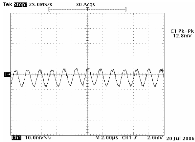
Figure 7: Output Ripple & Noise
