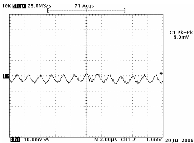
Figure 9: Output Ripple & Noise
