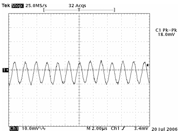
Figure 11: Output Ripple & Noise
