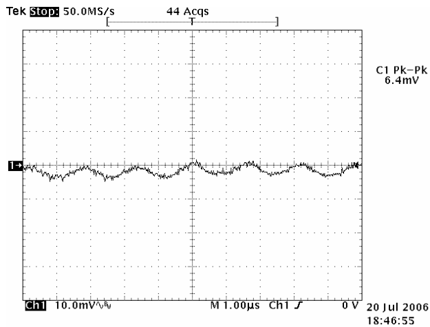
Figure 1: Output Ripple & Noise ( V_{in}=2.97V , V_{out}=0.59V/10A , Environment Temp= 25^{\circ}C )
