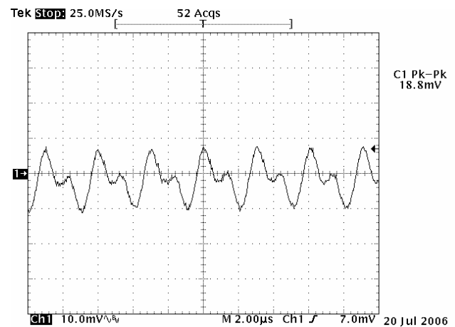
Figure 10: Output Ripple & Noise
