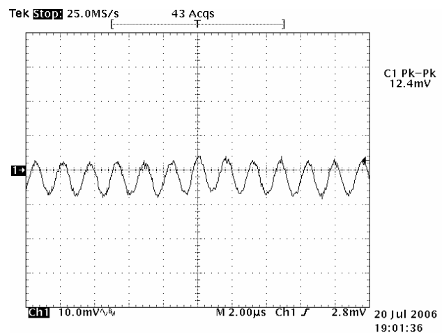
Figure 6: Output Ripple & Noise ( V_{in}=5.5V , V_{out}=2.5V/10A , Environment Temp= 25^{\circ}C )
