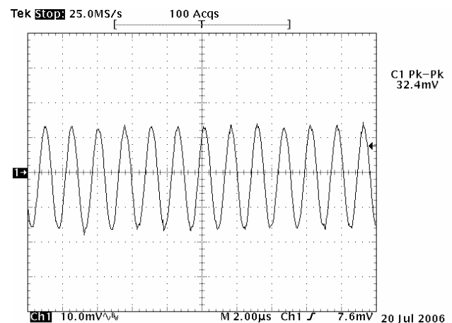
Figure 12: Output Ripple & Noise
