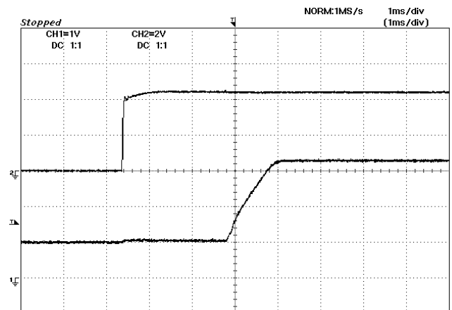
Figure 26: Typical transient response to step load change at 2.5A/μS from 50% to 100% of I_o , max at 3.3Vin, 1.8Vout (Cout = 1μF ceramic, 10μF tantalum)
