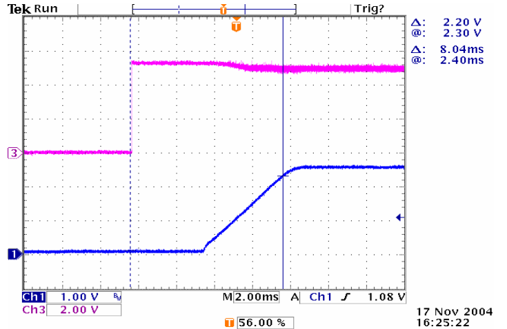
Figure 18: Turn on delay time at remote turn on with external capacitors (Co= 5000 μF) 3.3Vin, 2.5V/16A out
