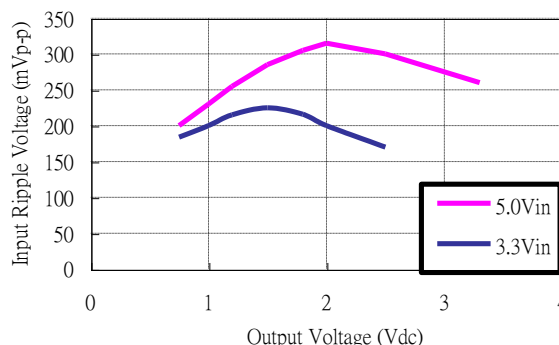
Figure 32: Input voltage ripple for various output models, I_O = 16 A ( C_{IN} = 2 \times 100 \mu\text{F} tantalum // 47 \mu\text{F} ceramic)
