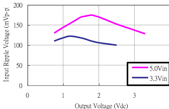
Figure 33: Input voltage ripple for various output models, I_O = 16 A ( C_{IN} = 4 \times 100 \mu\text{F} tantalum // 2 x 47 \mu\text{F} ceramic)
