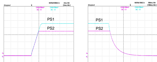
Figure 40: Sequential Start-up
