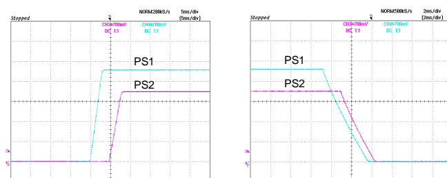
Figure 40: Sequential Start-up
