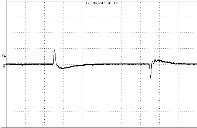
Figure 35: Typical transient response to step load change at 1A/\mu S from 0%~ 50%~0% of I_o , max at 12V_{in} , 3.3V_{out} ( C_{out} = 1\mu F ceramic, 47\mu F + 10\mu F ceramic) CH1 : V_{OUT} , 0.2V/div, 100 \mu S /div
