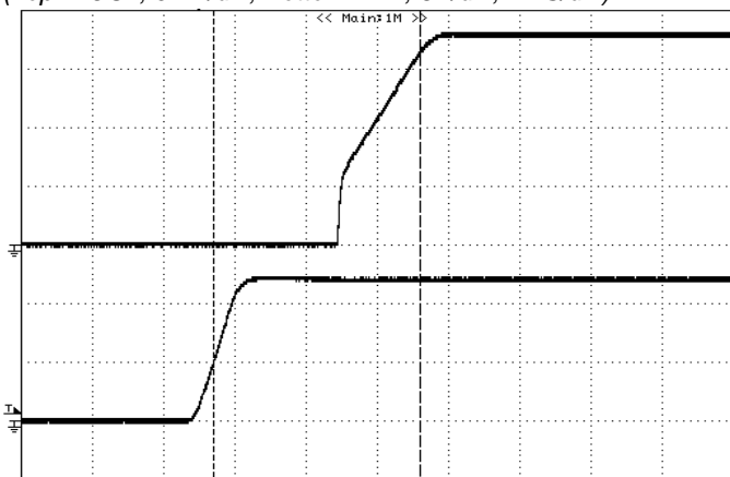
Figure 15: Turn on delay time at 12Vin, 1.8V/12A out. (Top: VOUT, 0.5V/div; Bottom: VIN, 5V/div; 2mS/div)
