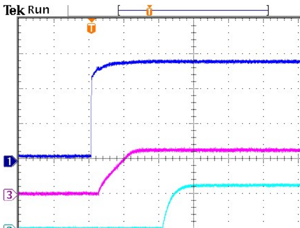
Figure 15: Control turn on at 12Vin, 2.5V /20A Ch1: Enable, Ch3: Vo, Ch2: PG
