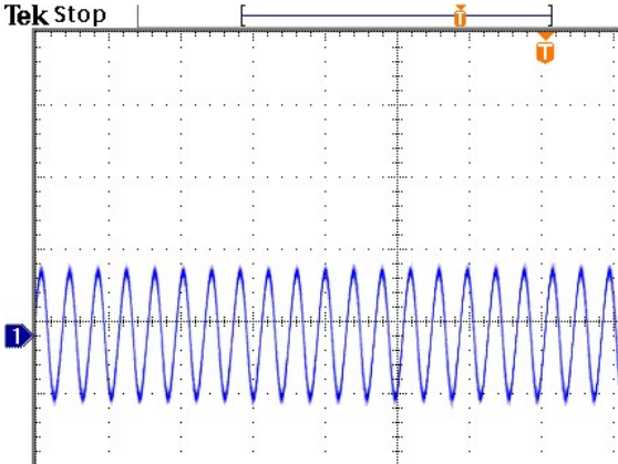
Figure 8: Output ripple & noise at 12Vin, 3.3V/20A out
