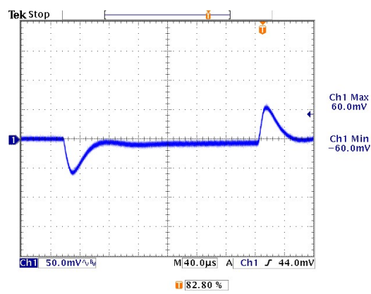
Figure 20: Transient response, 3.3V /20A, Ch1: Vo
