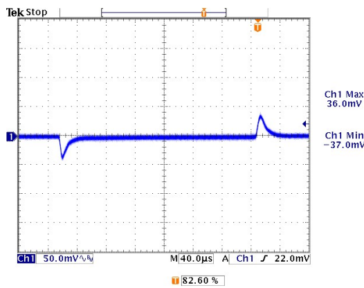
Figure 22: Transient response, 1.5V /20A, Ch1: Vo
