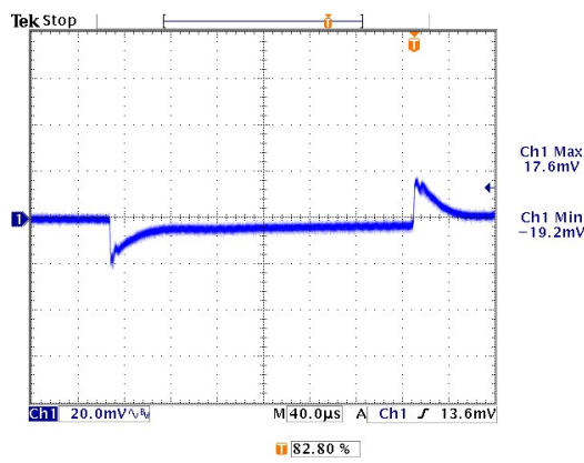
Figure 24: Transient response, 0.9V /20A, Ch1: Vo
