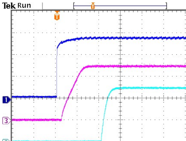
Figure 13: Control turn on at 12Vin, 5.0V /20A Ch1: Enable, Ch3: Vo, Ch2: PG
