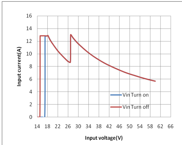
Figure 7: Input current vs. Input voltage @ V_{in}=18V\sim27V , 200W; V_{in}=27V\sim60V , 300W
