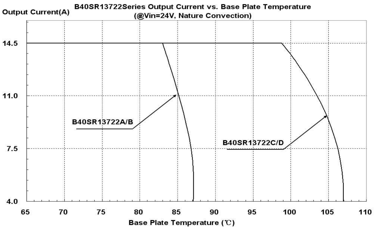
Figure 21: Output Current vs. Base Plate temperature @Vin=24V
