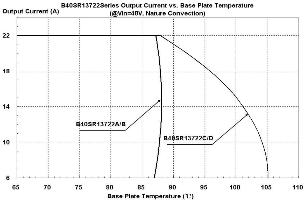
Figure 23: Output Current vs. Base Table temperature @ Vin=48V
