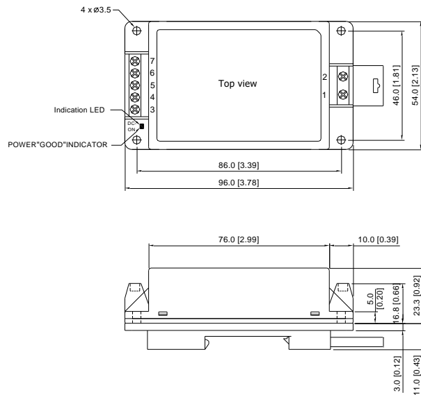
Mechanical Dimensions
