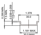
SUGGESTED DIMENSION OF DIN RAIL
