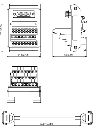
ACS3-MDTD2600 (for B3-M, F, and E)
