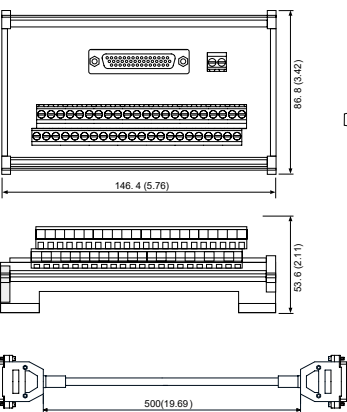
ACS3-MDTB4400 (for B3-L)
