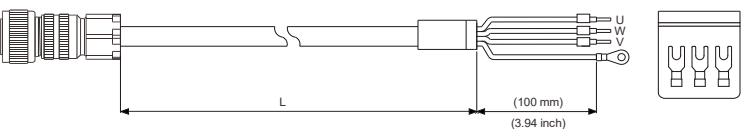
F180, 2/3/4.5kW B3 motor, w/o brake, straight connector
