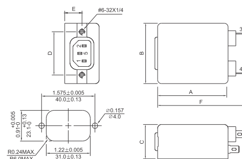
SUGGESTED MOUNTING CUTOUT
