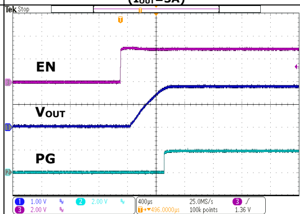
FIGURE 14 Turn-On (V IN =3.3V, I OUT =3A)
