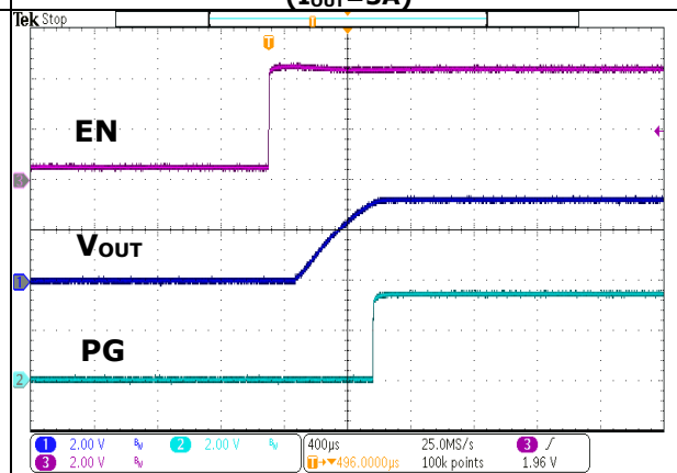
FIGURE 8 Turn-On (V IN =5.0V, I OUT =3A)
