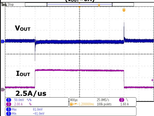
FIGURE 7 Transient Response (V IN =5.0V, I OUT =0.3A~3A)
