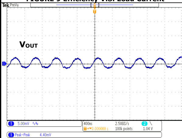
FIGURE 11 Output Ripple at 3.3V IN (I OUT =0A)
