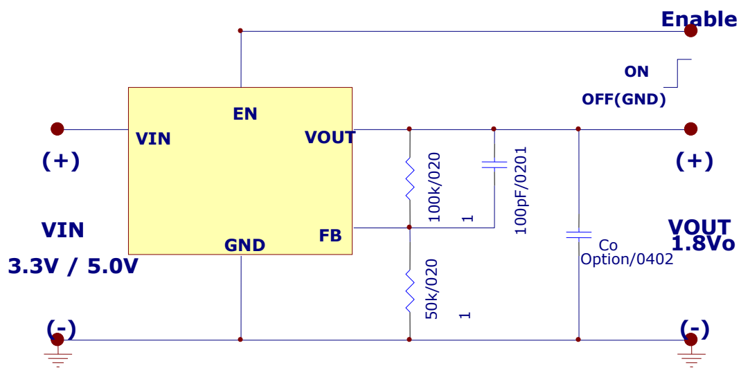
FIG.39 TYPICAL APPLICATION FOR PWM OPERATION
