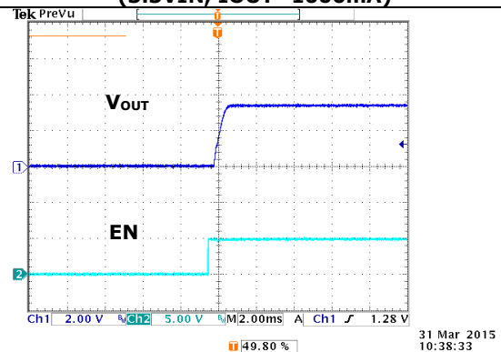
FIG.38 TURN-ON (3.3VIN, IOUT=1000mA)
