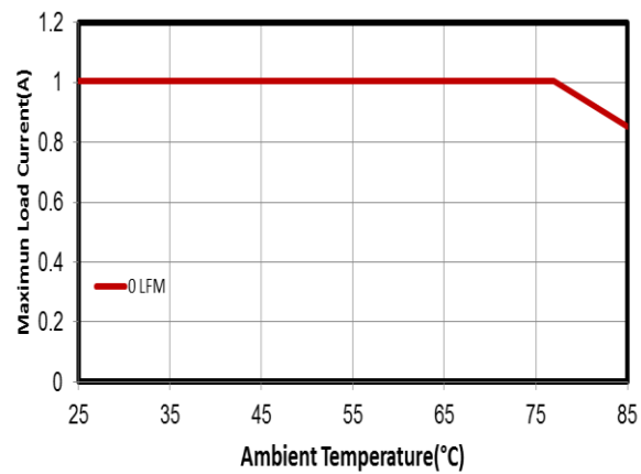
FIG.34 DE-RATING CURVE AT 5.0VIN
