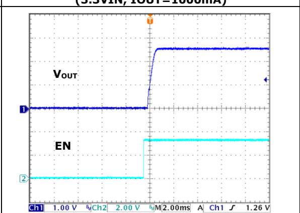
FIG.32 TURN-ON (3.3VIN, I_{OUT}=1000\text{mA} )
