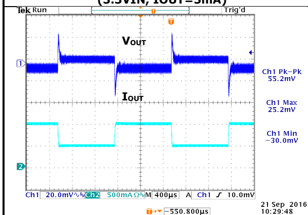
FIG.31 TRANSIENT RESPONSE (5.0VIN, 50% to 100% LOAD STEP)
