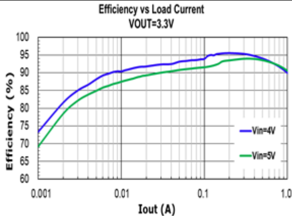
FIG.33 EFFICIENCY V.S. LOAD CURRENT
