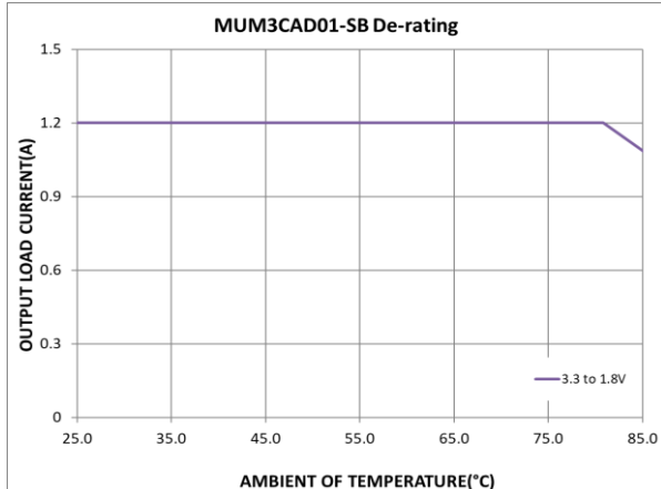
FIG.22 DE-RATING CURVE AT 3.3VIN
