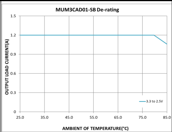
FIG.28 DE-RATING CURVE AT 3.3VIN
