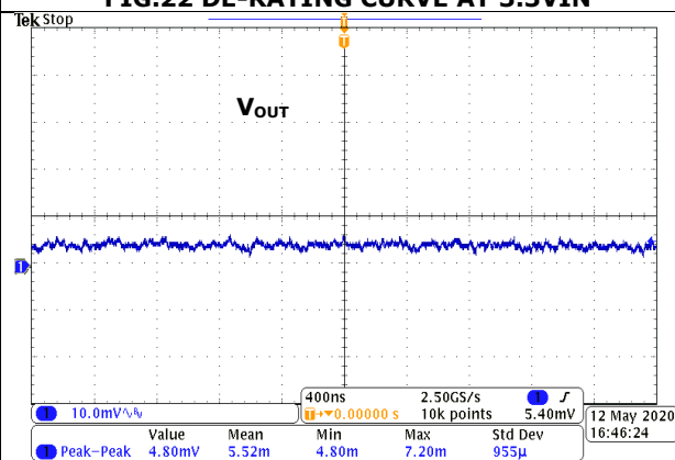
FIG.24 OUTPUT RIPPLE (3.3VIN, IOUT=1000mA)
