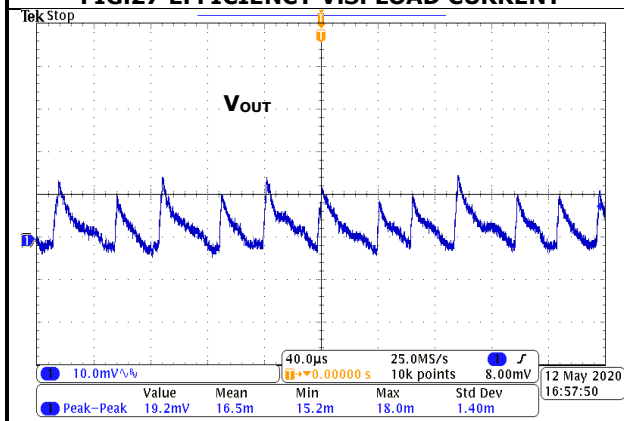
FIG.29 OUTPUT RIPPLE (3.3VIN, I_{OUT}=5\text{mA} )
