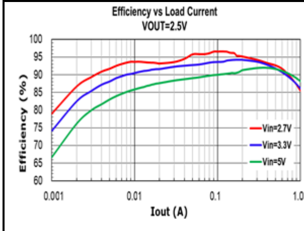
FIG.27 EFFICIENCY V.S. LOAD CURRENT
