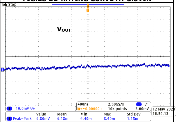
FIG.30 OUTPUT RIPPLE (3.3VIN, I_{OUT}=1000\text{mA} )
