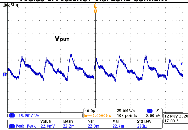
FIG.35 OUTPUT RIPPLE (5.0VIN, IOUT=5mA)
