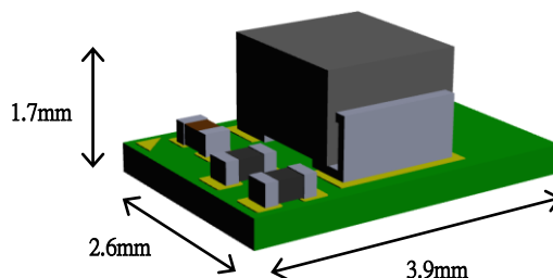
FIGURE.2 HIGH DENSITY uPOL MODULE
