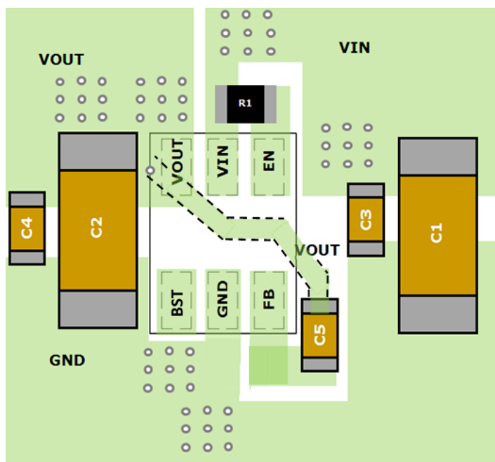
FIG.19 PCB LAYOUT
