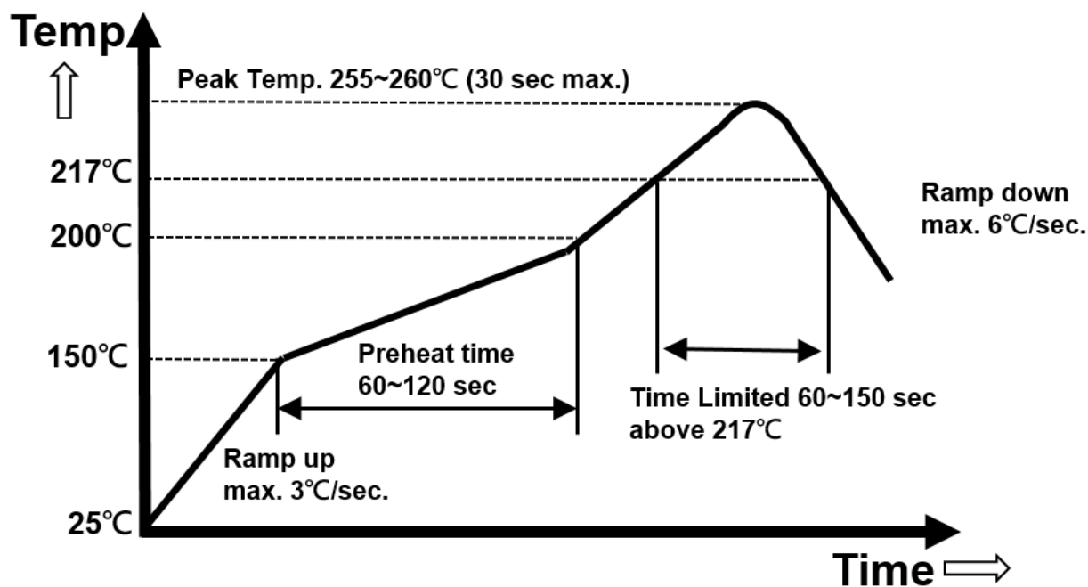
FIG.21 Recommendation Reflow Profile (Not to scale)
