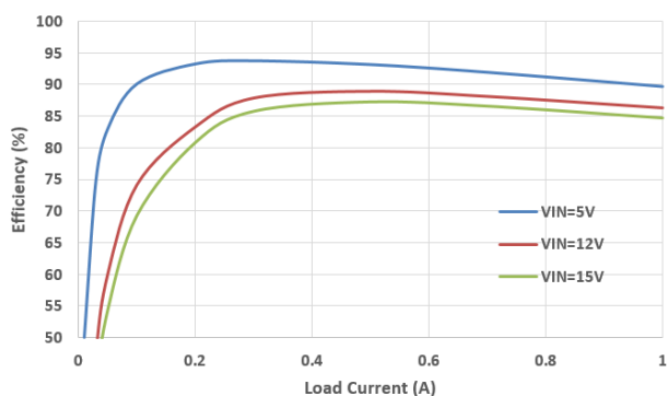
FIG.3 EFFICIENCY V.S. LOAD CURRENT
