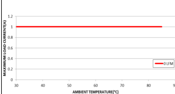
FIG.4 DE-RATING CURVE AT VIN=12V
