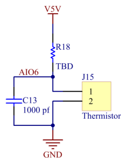
Figure 6 External Thermistor Circuitry
