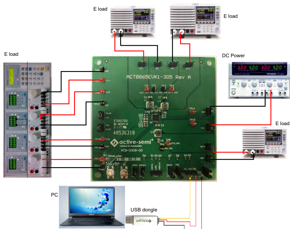
Figure 2 – EVK Setup
