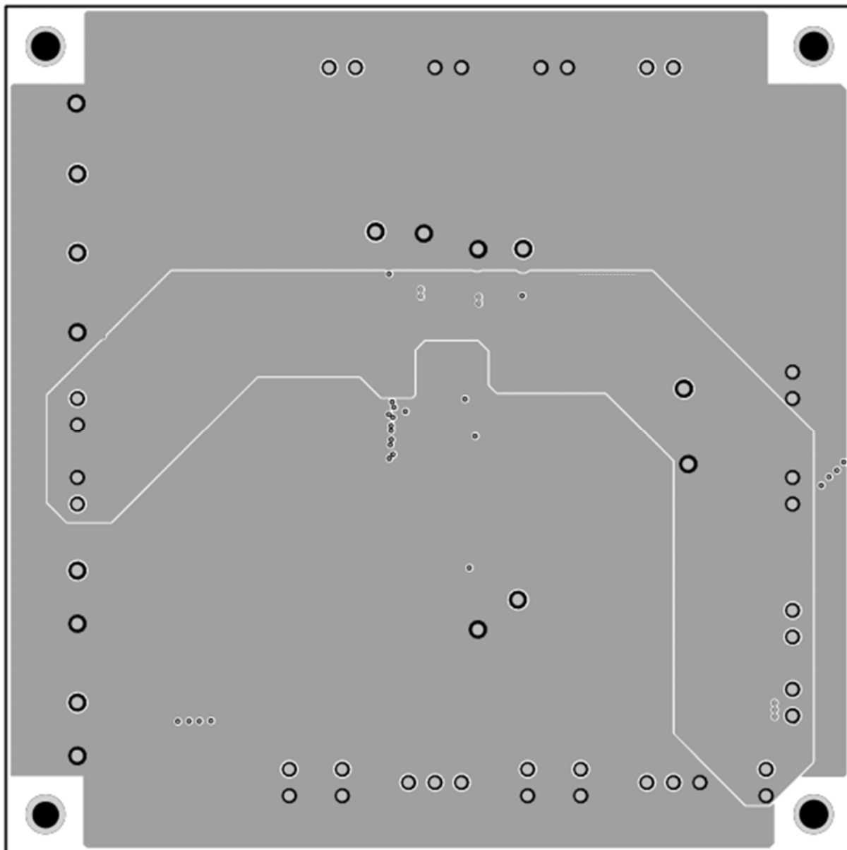
Figure 7 – Layout Layer 2
