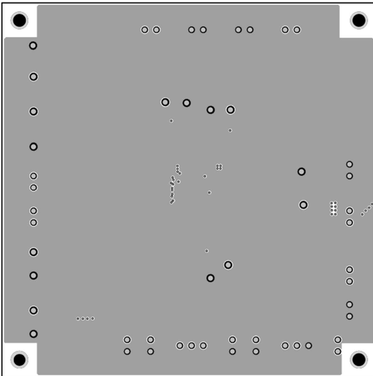
Figure 7 – Layout Layer 3
