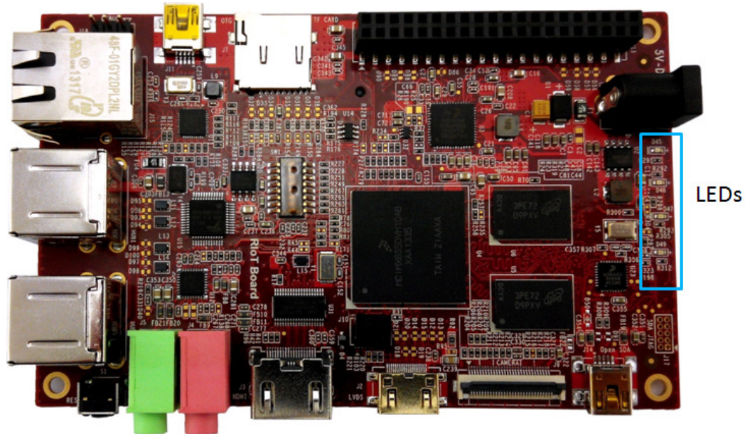
Figure 2-20 LEDs
