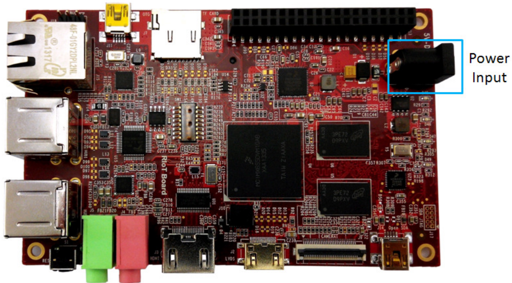
Figure 2-2 Power Interface
