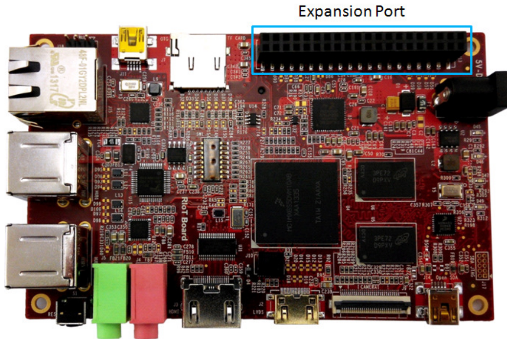
Figure 2-14 Expansion Port
