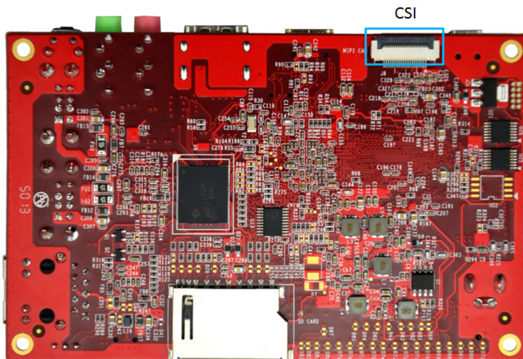
Figure 2-9 CSI Interface
