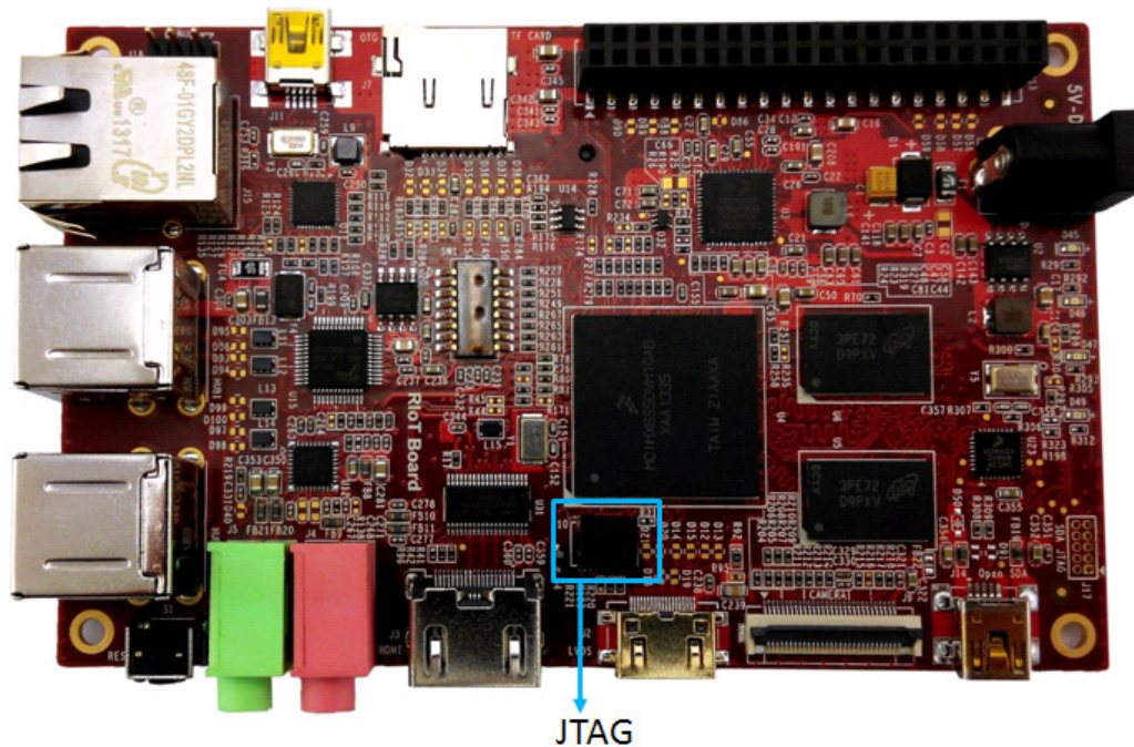
Figure 2-11 JTAG Interface
