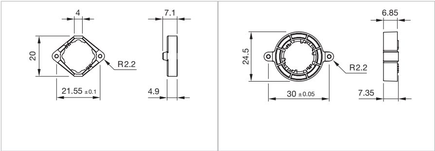
Dimensions [mm] for Part No. 92-960.0 Dimensions [mm] for Part No. 84-960.0
