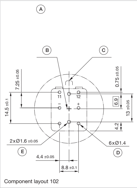
Dimensions [mm] A = Drilling plan (component side) B = Centre from switch C = Anti-twist protection D = Pins for contacts/LED E = Positioning hole
