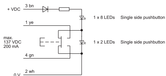
Wiring diagram 1
