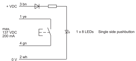
Wiring diagram 2
