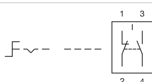
Wiring diagram 120
