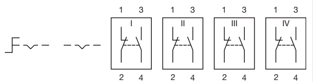
Wiring diagram 127
