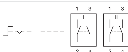
Wiring diagram 121
