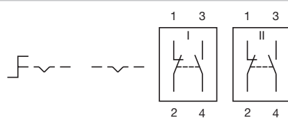
Wiring diagram 118
