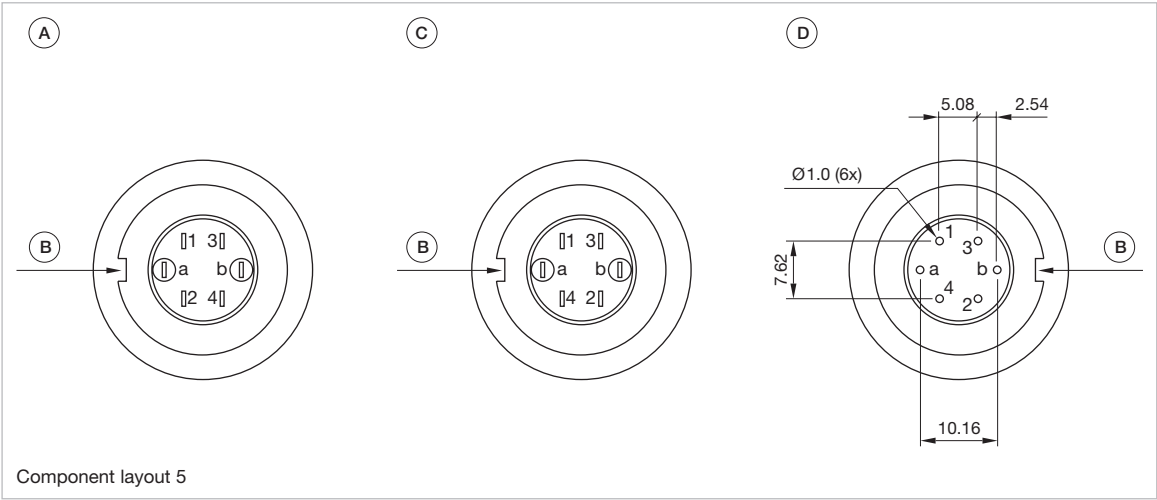
Dimensions [mm] A = Terminals (rear side) B = Anti twist device C = Diode block D = Drilling plan (component side)
