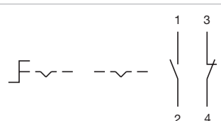
Wiring diagram 117
