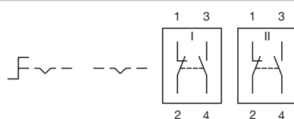
Wiring diagram 118
