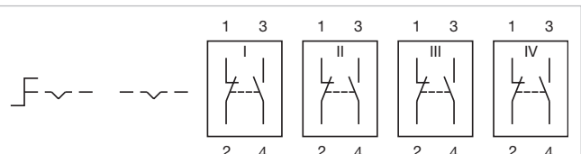
Wiring diagram 124
