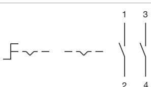
Wiring diagram 123
