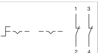
Wiring diagram 118
