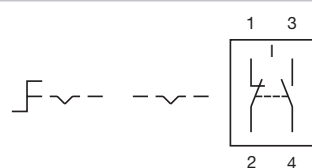
Wiring diagram 117
