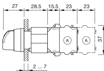
Dimensions [mm] A = Screw terminal
