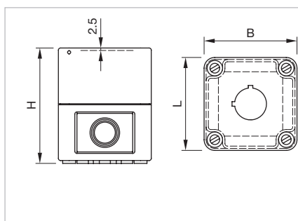
Dimensions [mm]
