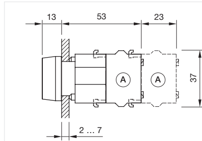
Dimensions [mm] A = Screw terminal
