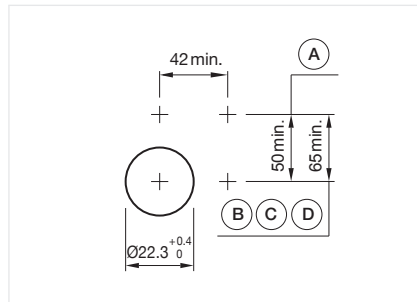
Mounting cut-outs [mm] A = Screw terminal B = Push-in terminal (PIT) C = Plug-in terminal 6.3 mm x 0.8 mm D = Double plug-in terminal 6.3 mm x 0.8 mm
