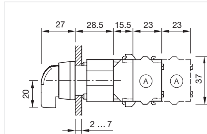
Dimensions [mm] A = Screw terminal
