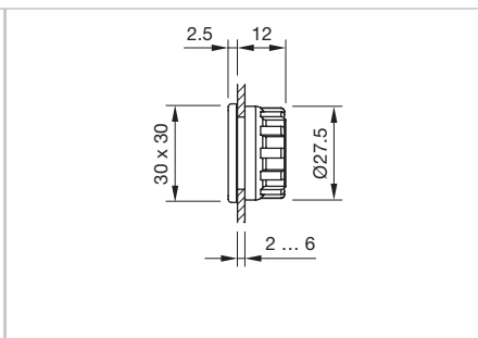
Dimensions [mm] for Part No. 704.964.7
