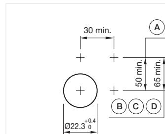
Dimensions [mm] A = Screw terminal
