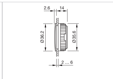
Dimensions [mm] for Part No. 704.964.8
