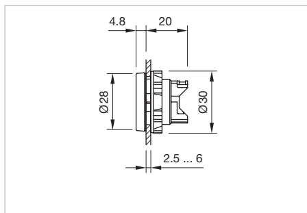
Dimensions [mm] for Part No. 704.960.4
