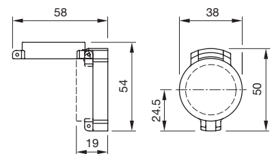
Dimensions [mm] for Part No. 704.928.28, 704.928.38
