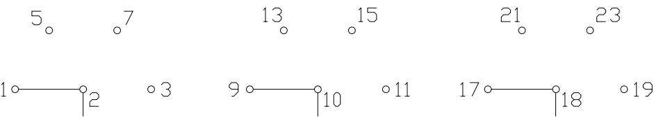
12 rotary selector switch element 60° page 103
