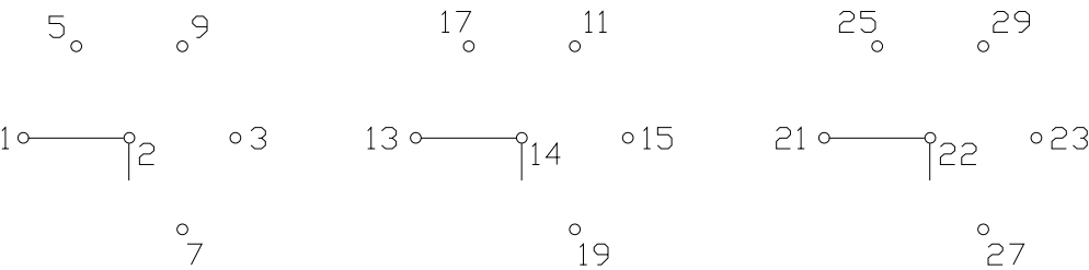
15 rotary selector switch element 60° page 103
