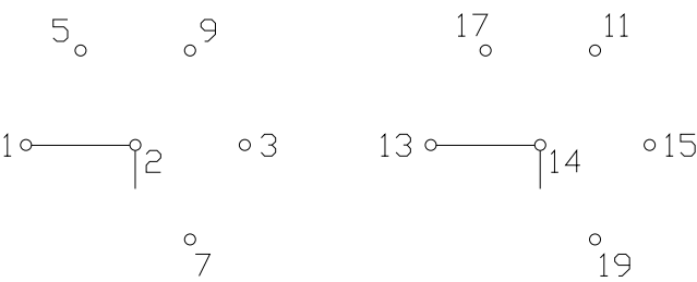
15 rotary selector switch element 60° page 103
