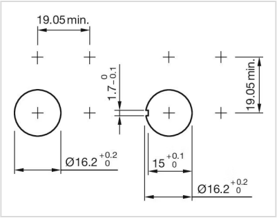
Dimension drawings:
