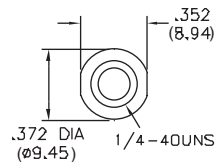
Dress Nut
