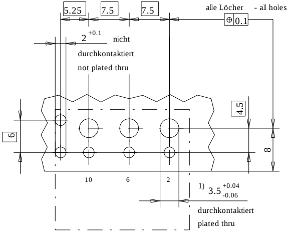
Board hole pattern (Component mounting side) for high current contacts with press-fit termination
